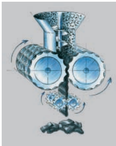
Compaction of aluminium chips and turnings, test in Köppern's pilot plant
